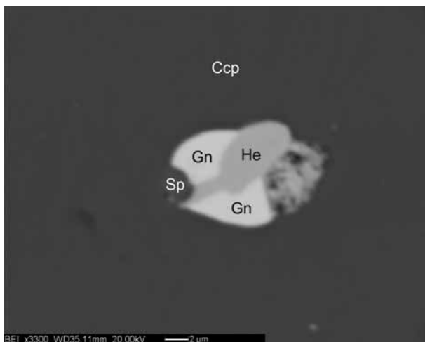
Fig. 24. Chalcopyrite (Ccp) including a polyminerallitic aggregate of galena (Gn), hessite (He) and sphalerite (Sp).
