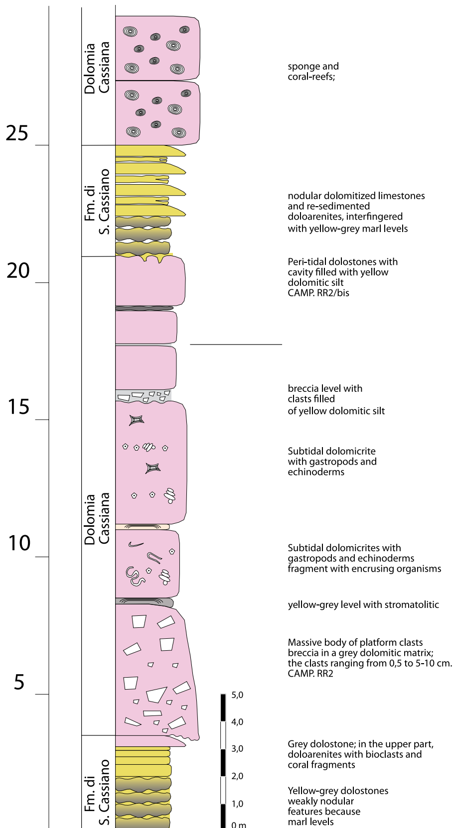
Fig. 10: The base of the Richt-hofen Reef (DC 1a) represents a carbonate wedge overlying the basin deposits with an erosional base (San Cassiano Fm). Note the details of the stratigraphic section.
