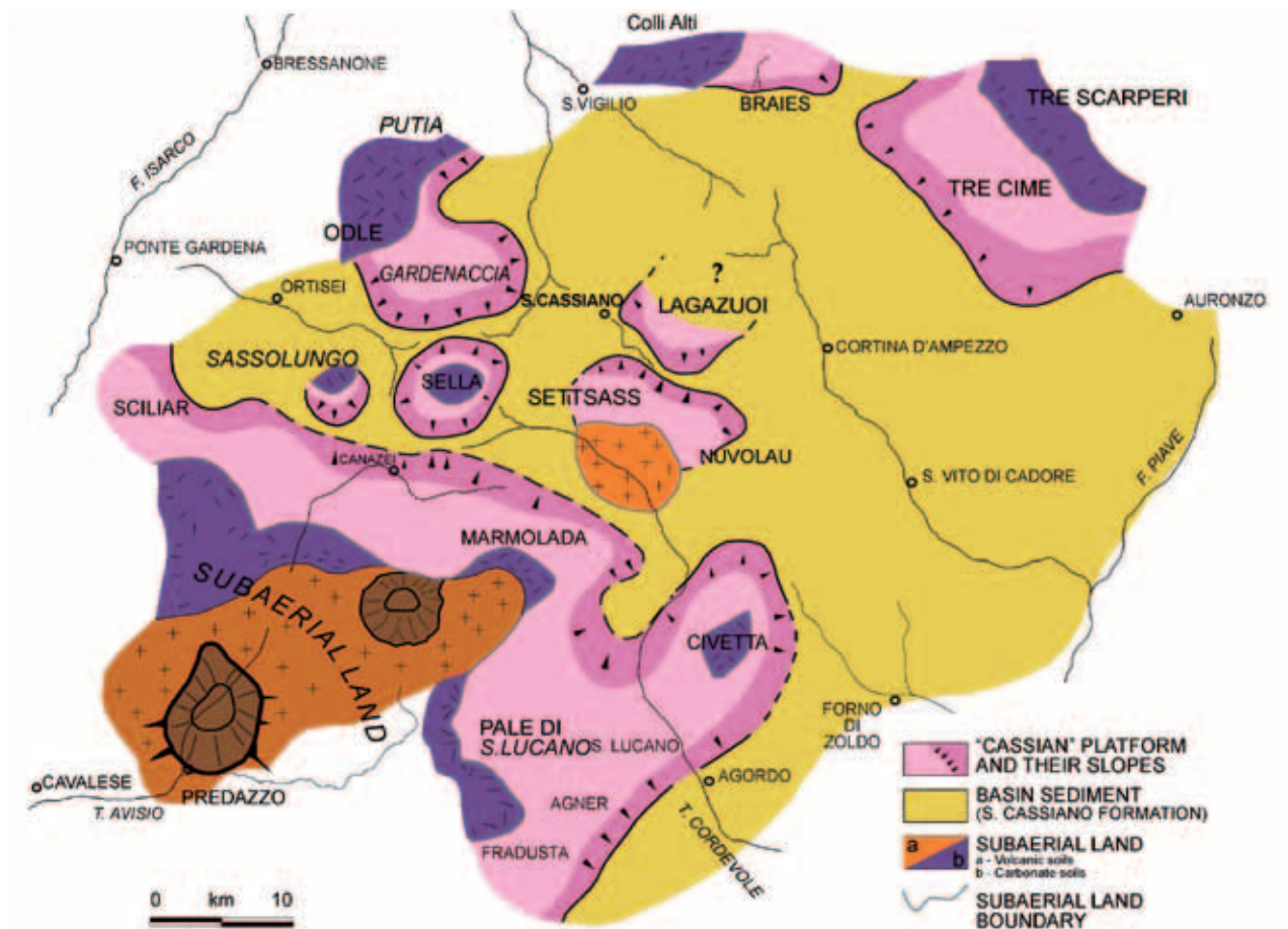
Fig. 4: Palaeogeographic map representing schematically the distribution of post-volcanic Triassic carbonate platforms of the Dolomites region and the spatial relationships with the Predazzo and the Monzoni volcanic edifices (redrawn after Bosellini, 1996).
